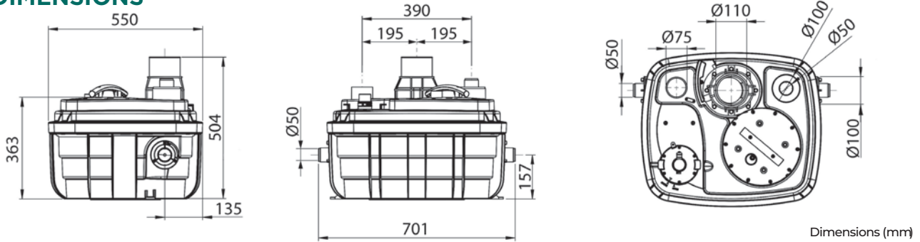
Dimensions (mm)
